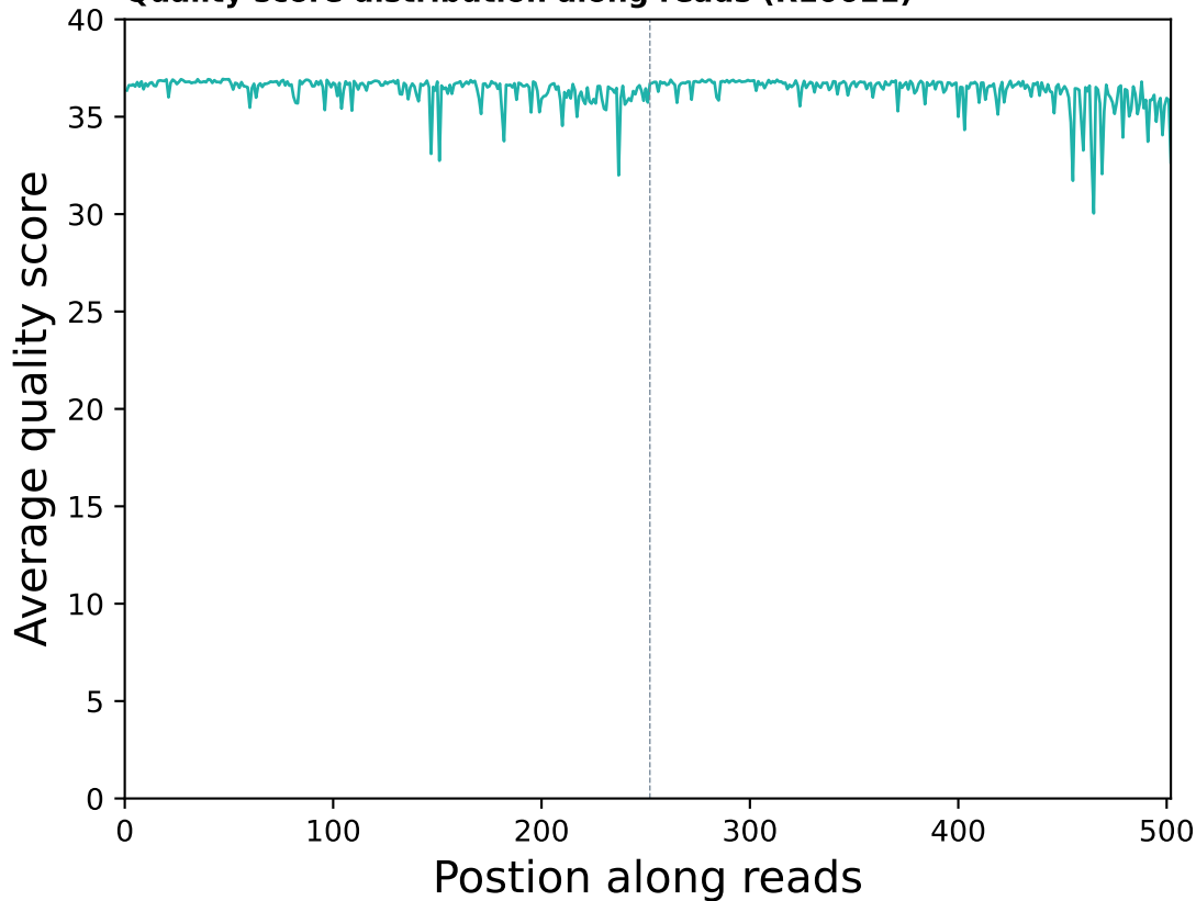
Quality score distribution along reads (R10611)
